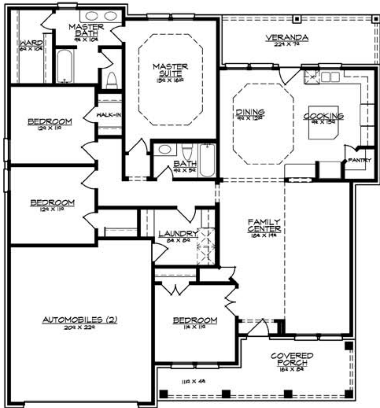
FLOOR PLAN
